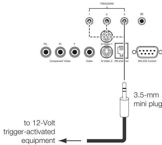
Figure 3-10. Connecting 12-Volt Trigger Outputs
